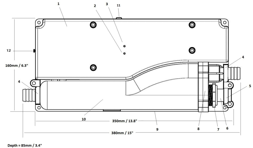
Parts Diagram:
